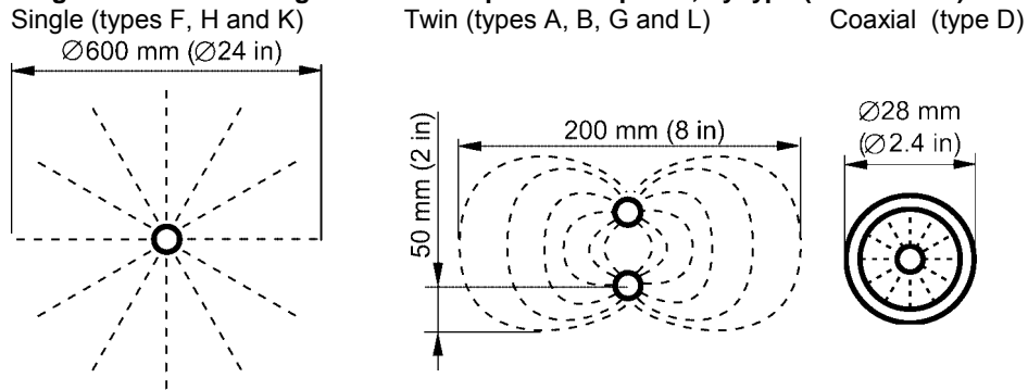
Diagram 12: Electromagnetic field shape around probe, by type (not to scale)
